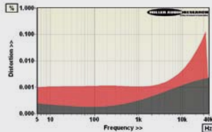
ABOVE: Distortion vs. frequency showing analogue preamp (black) vs. digital input at 96kHz/24-bit (red)
